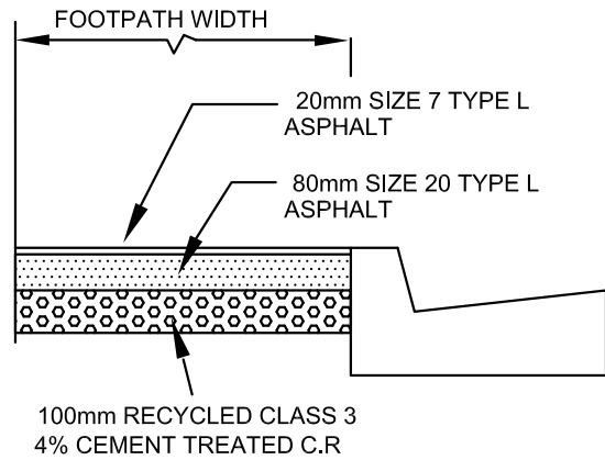
INDUSTRIAL ASPHALT FOOTPATH (IAF)
