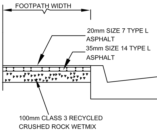
RESIDENTIAL ASPHALT FOOTPATH (RAF)
