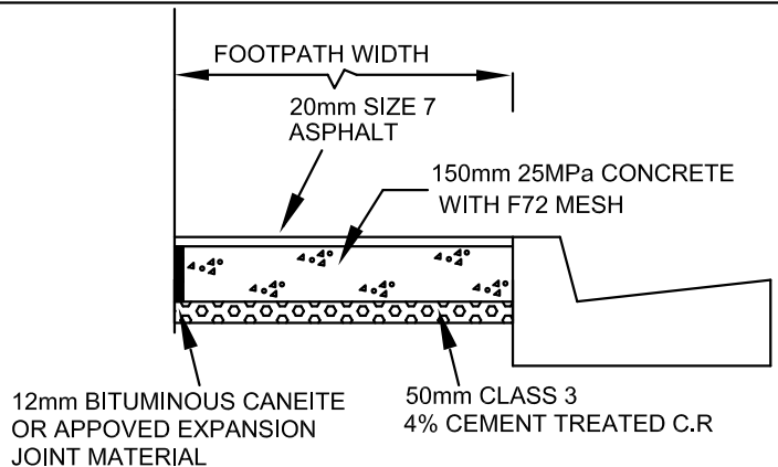
INDUSTRIAL CONCRETE FOOTPATH WITH ASPHALT SURFACE (ICAF)
