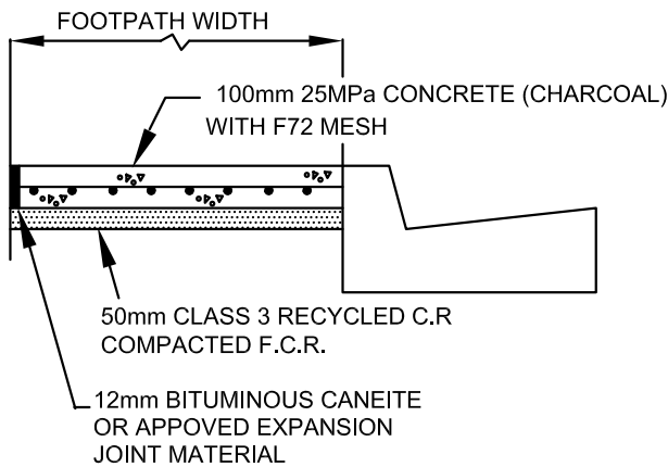
CONCRETE FOOTPATH (CF)
