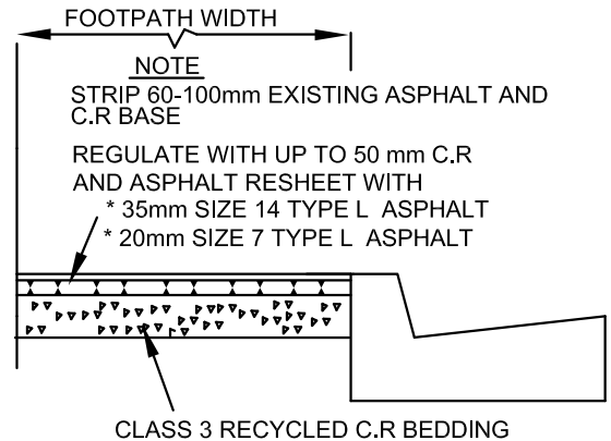
RESIDENTIAL FOOTPATH STRIP AND RESHEET
