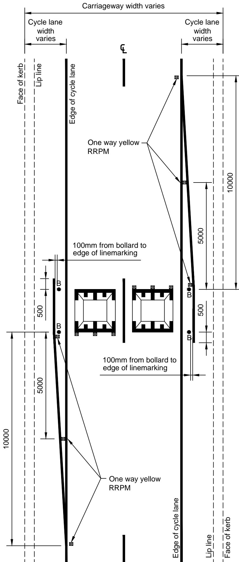
Plan Scale 1:100
